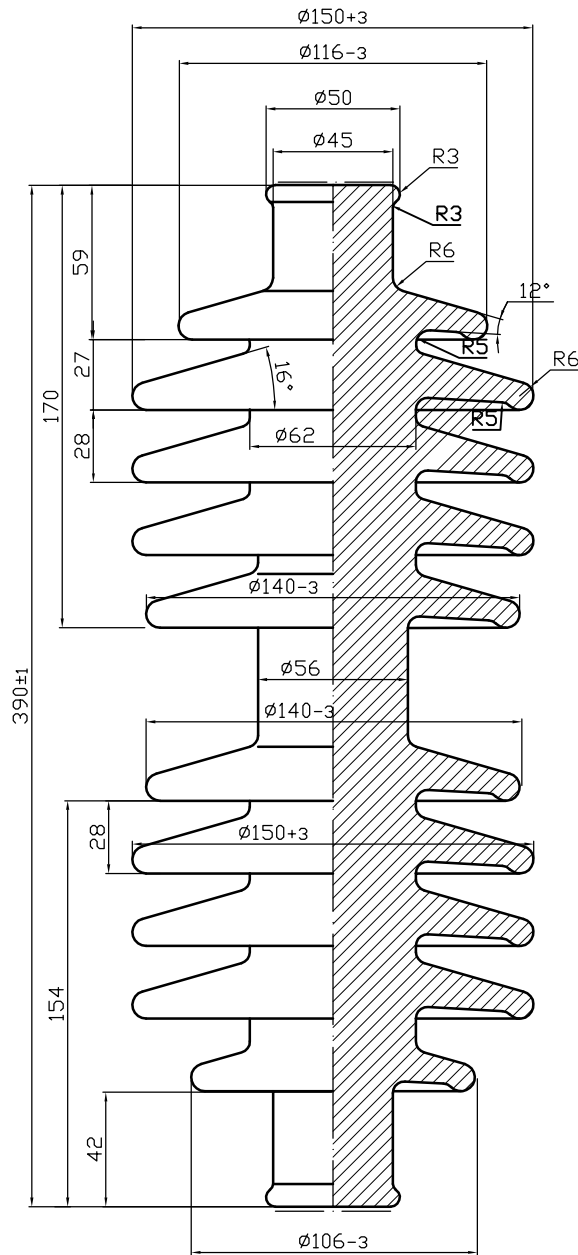
SỨ CẦU CHÌ 24KV(SCR24.EMIC) 24KV PUSE CUT-OUT INSULATORS (SCR24.EMIC)
