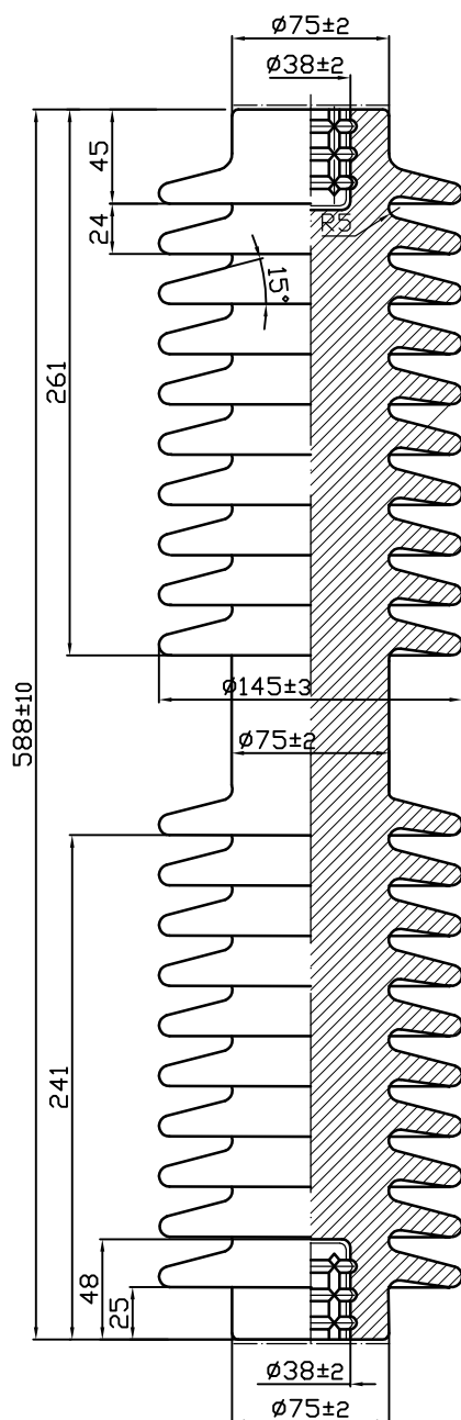
SÚ CẦU CHÌ 35KV(SCR35.CD875.VL) 35KV PUSE CUT-OUT INSULATORS (SCR35.CD875.VL)
